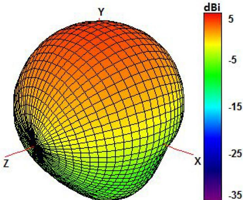
1575 MHz Radiation pattern
